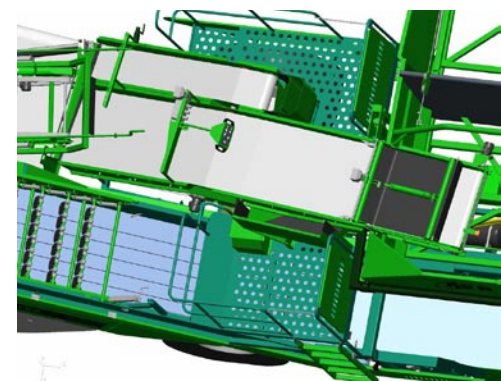
Flat picking-off table with large platform
